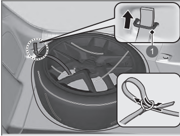
1 Rear Anchorage
