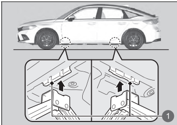
1 Jacking Points
